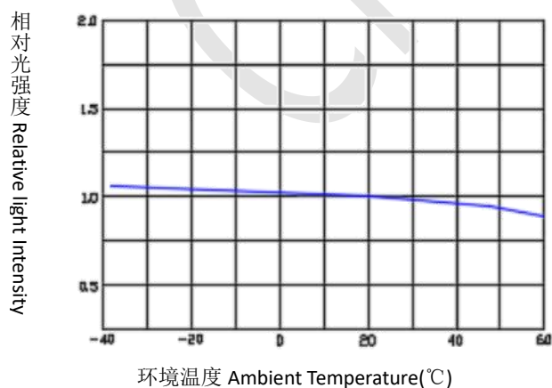
Relative Light Intensity vs. Ambient Temperature
