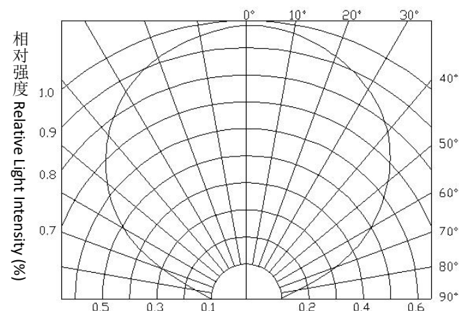
Relative Light Intensity vs. Angular Displacement
