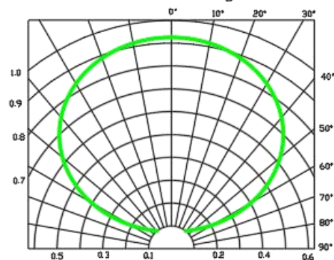
Radiation angle
