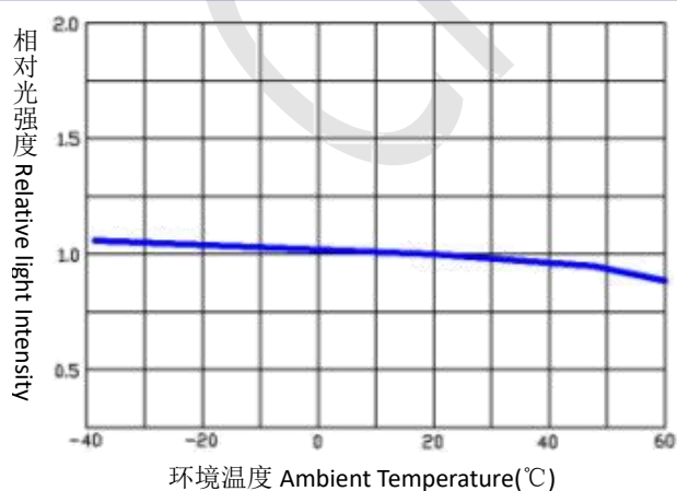
Relative Light Intensity vs. Ambient Temperature
