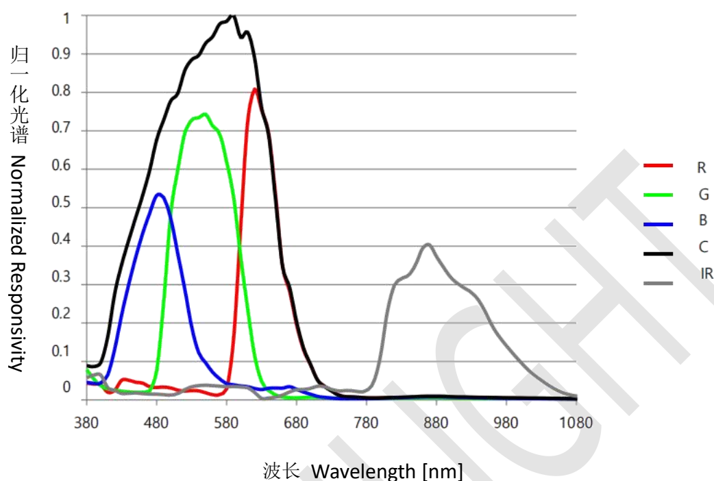
归一化相应曲线 Normalized Spectral Response
