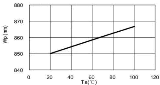
Fig.5-Peak Wavelength (@350mA) vs. Ambient Temperature
