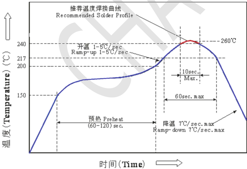
推荐回流焊曲线 Recommended Reflow Welding Curves
