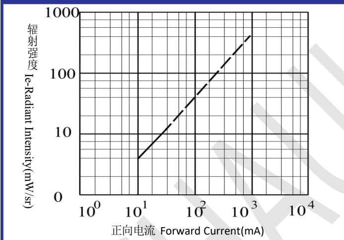
Radiant Intensity vs. Forward Current
